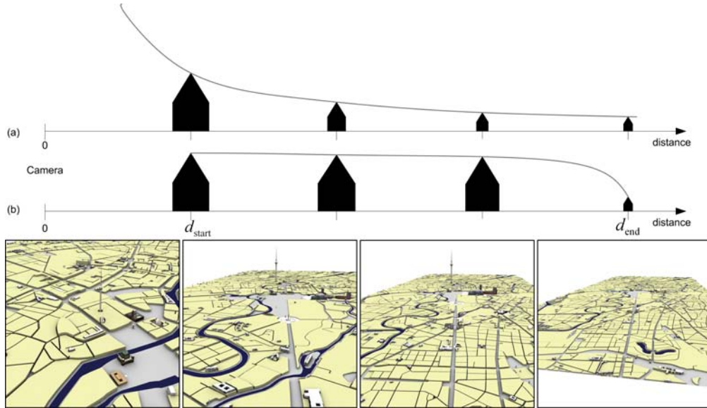
Figure 6: The traditional perspective projection (a) scales objects inversely proportional to the distance. Our scaling (b) keeps the size of the landmark object nearly constant within a distance interval and blend smoothly to the original scaling at the interval limits. Note how the dynamic landmarks, e.g., the TV tower, keep their projected size while departing it, until the end distance is reached (screenshots).
